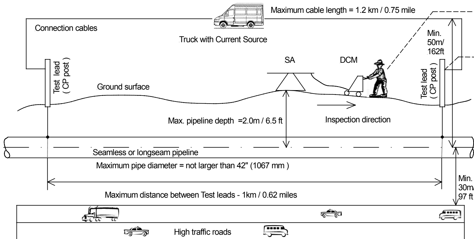
Schematic presentation of the NoPig inspection. The NoPig inspection tool contains 2 modules: SA = Sensor Array and DCM = Data Collector Module. The pictures on the right show: (on the top) the NoPig Team during inspection; (in the middle) cable connection to the pipeline in a dig hole, and (at the bottom) cable connection to the pipeline in a CP-Post. The Right Of Way (ROW) over the pipeline must be accessible for putting the NoPig tool and be free from any obstacles.
